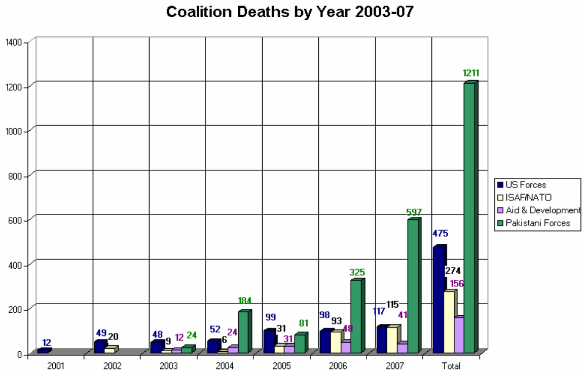
Figure 26. Coalition Deaths by Year 259
